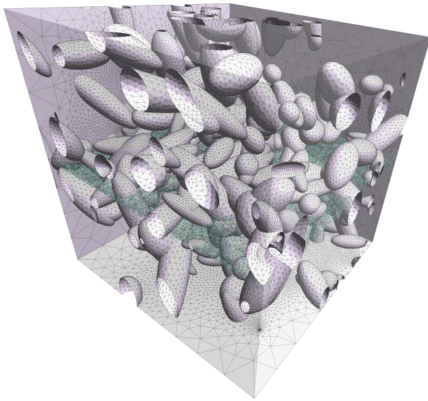
Figure 19: CAD model with 450 ellipsoids with random orientations and dimensions.
