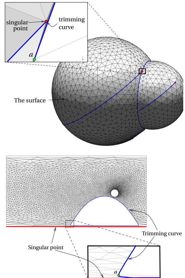
Figure 18: One surface of the 5000 sphere model that exhibit a complex configuration close to one of the poles of the sphere.
