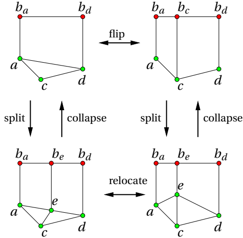
Figure 14: Local mesh modifications with irregular points.
