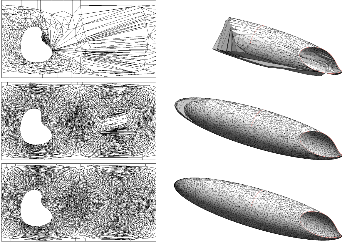
Figure 15: Different stages of the MeshAdapt algorithm
